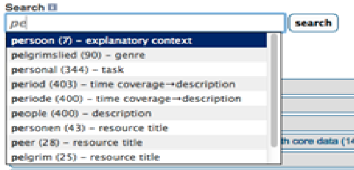
Figure 1a: Auto completion with hit count and contextual metadata information
