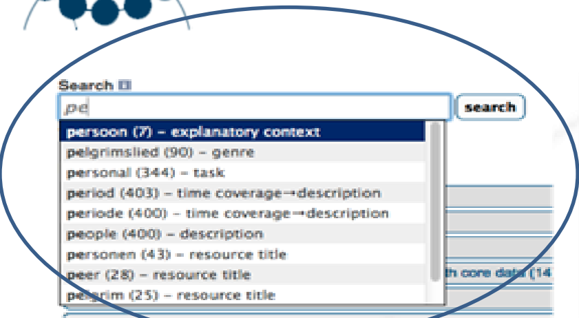
Figure 1a: Auto-completion with hit count and contextual metadata information
